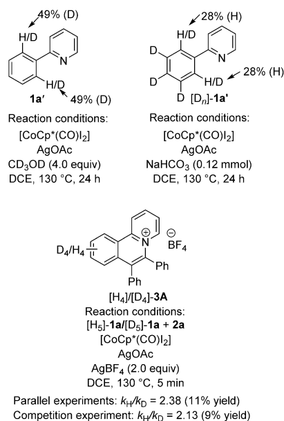
Scheme 4. Deuterium-labeling experiments.
